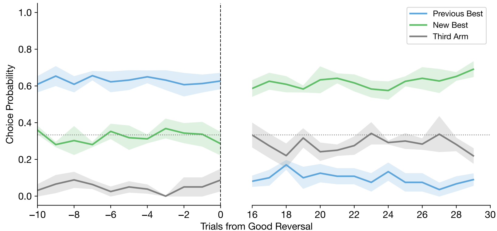
Good Reversal-Aligned Choices (mean \pm se across subjects | n=4 subjects, n=47 reversals) (Skipping first 15 trials post-reversal)
